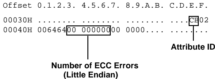
FIGURE 8: Number of ECC Errors Example
