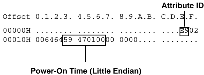
FIGURE 4: Power-On Time Example
