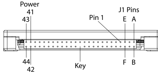
Figure 3: XceedSecure2 2.5" PATA Connection View
